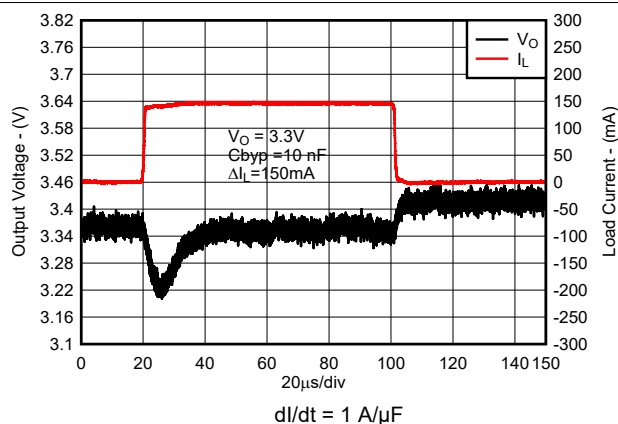
Figure 8-10. Load Transient for New Chip
